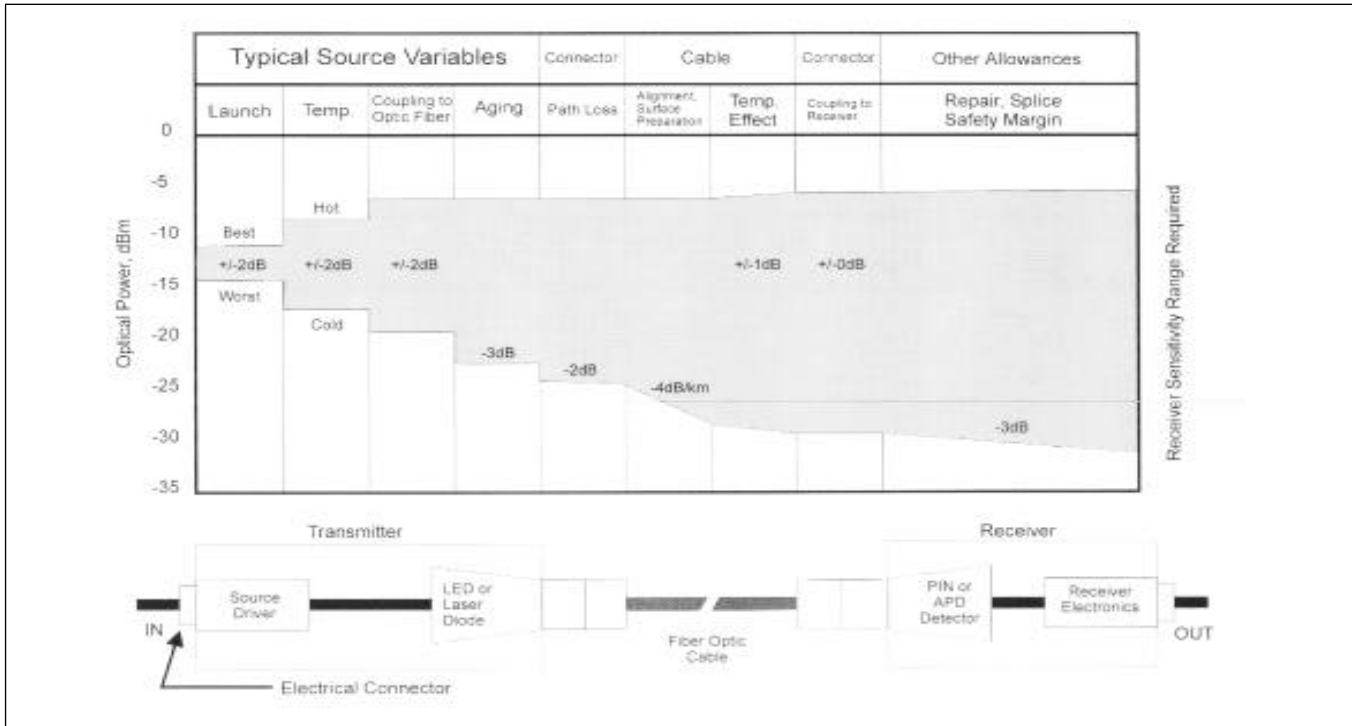
Figure 6. Optical link loss budget (courtesy of Force, Inc.).
