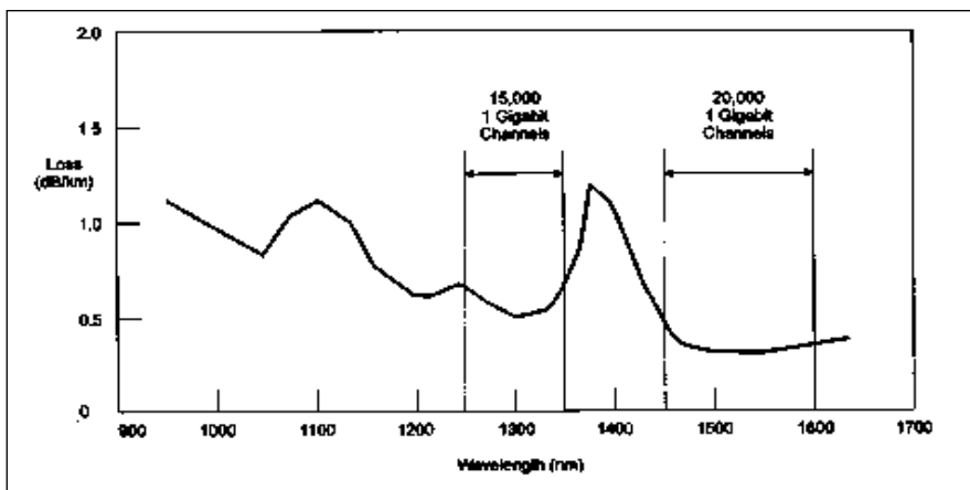
Figure 5. Bandwidth capacity of single-mode fiber.
