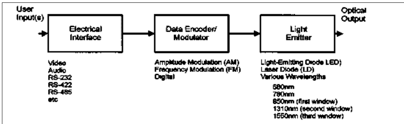
Figure 1. Fiber-optic transmitter (courtesy of Force, Inc.).
